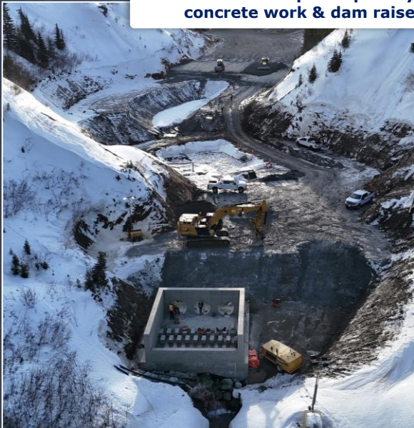
Sediment control pond spillway concrete work & dam raise
